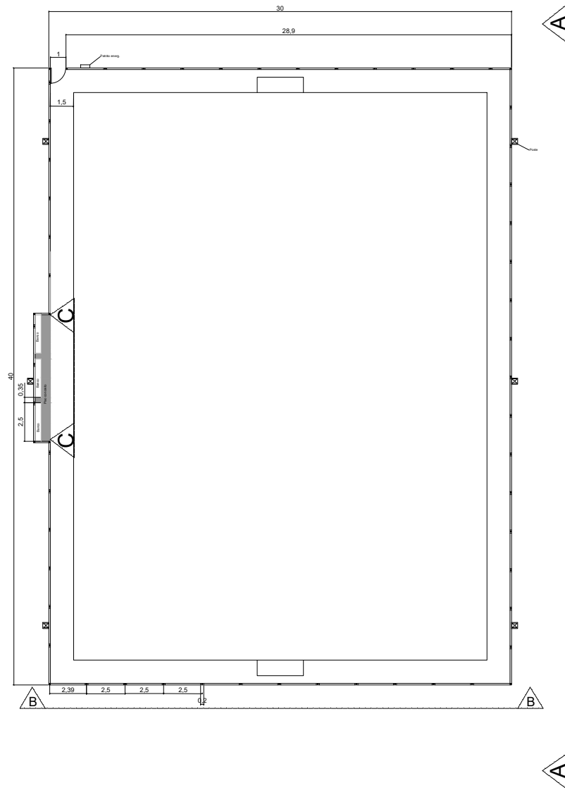
Vista frontal
